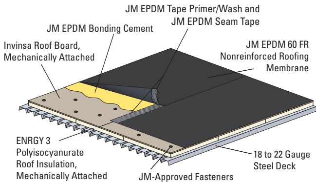
Fully adhered, nonreinforced JM EPDM single ply roofing system. For use over Johns Manville insulation, approved decks or other approved insulation on inclines up to 6 inches per foot (500 mm/m).
