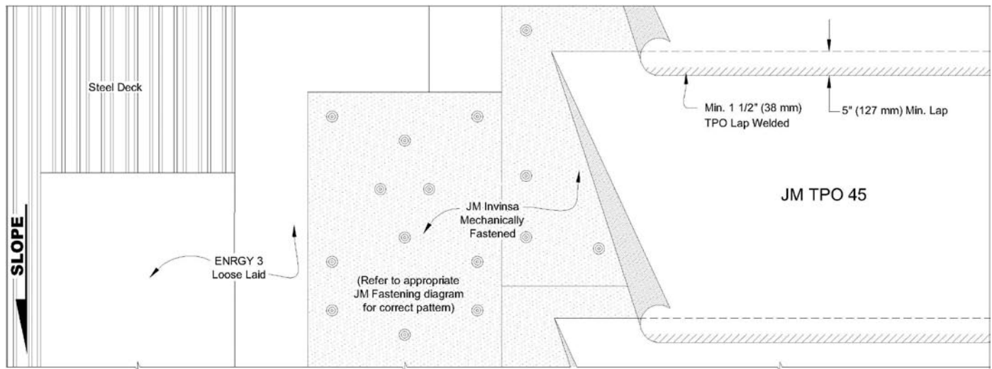
JM TPO 45 Mil Fully Adhered Membrane System Over ENRGY 3® Insulation and Invinsa™ Coverboard Fastened to a Steel Deck
