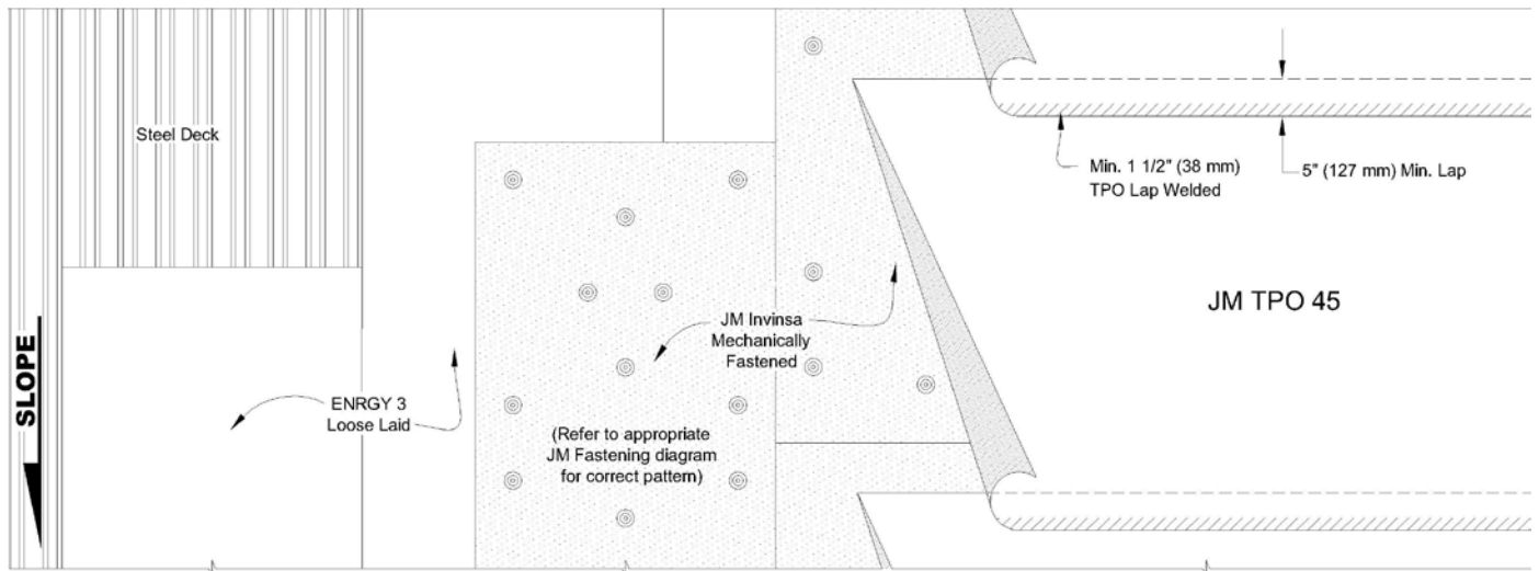
JM TPO 45 Mil Mechanically Fastened Membrane System Over ENRGY 3 ® Insulation and InvinSA ™ Coverboard Fastened to a Steel Deck
