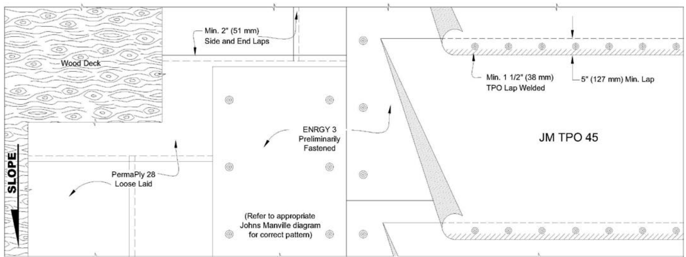
JM TPO 45 Mil Mechanically Fastened Membrane System Over ENRGY 3® Insulation and PermaPly® 28 Base Sheet Loose Laid on a Wood Deck
