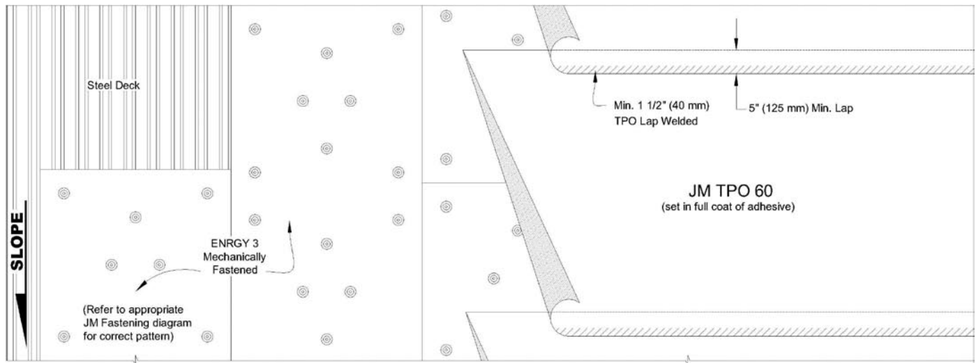
JM TPO 60 Mil Fully Adhered Membrane System Over ENRGY 3® Insulation Fastened to a Steel Deck
